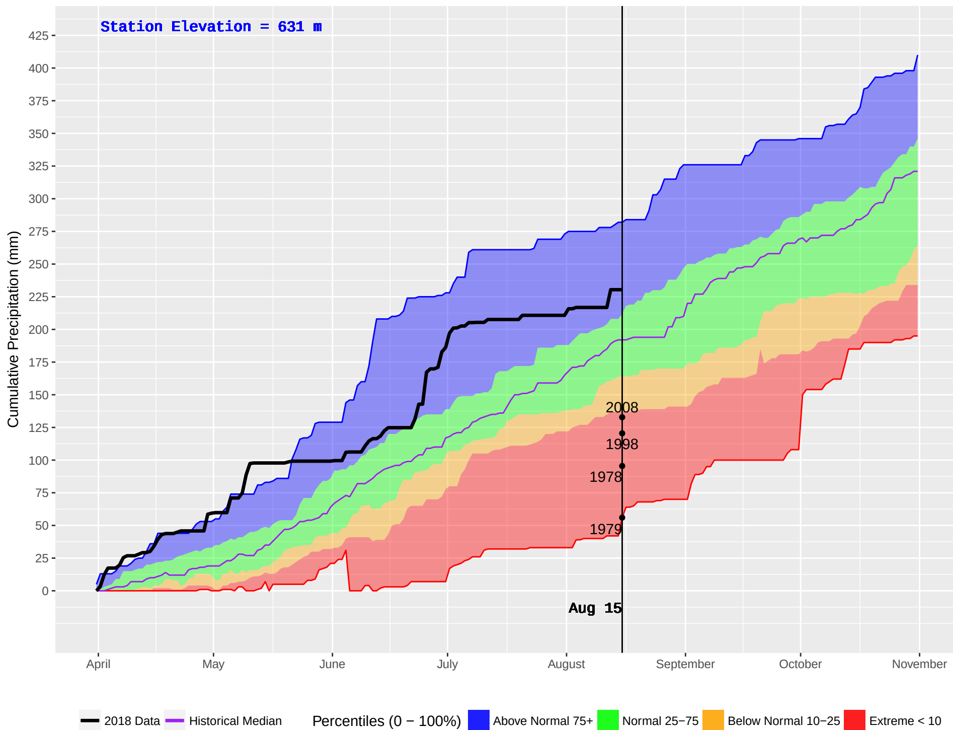
EAST BARRIERE (243) : Historical (1978–2016) and Current (2018) Daily Cumulative Precipitation
